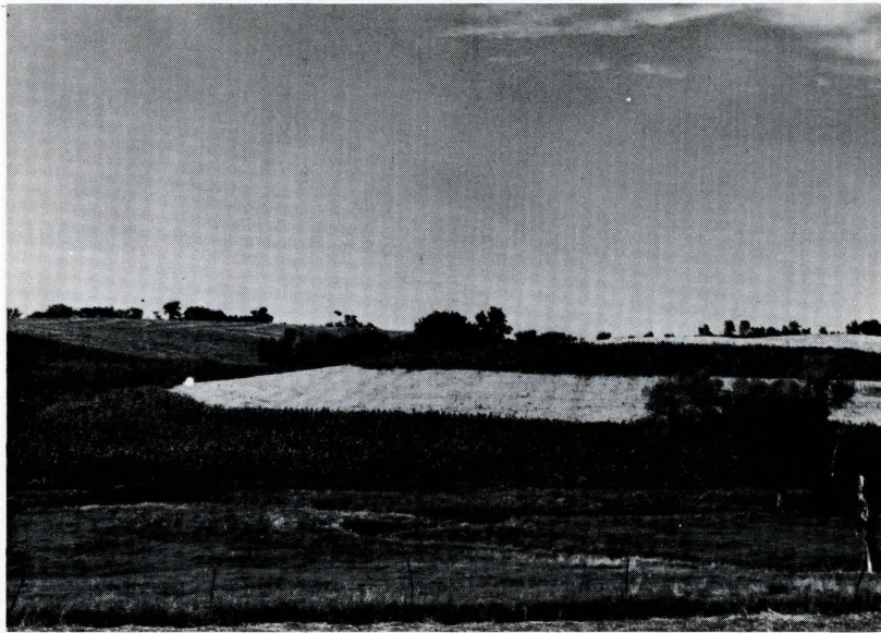
Strip cropping cuts soil losses to 1/4. LeRoy Simbro farm, Diamond Lake Watershed.
