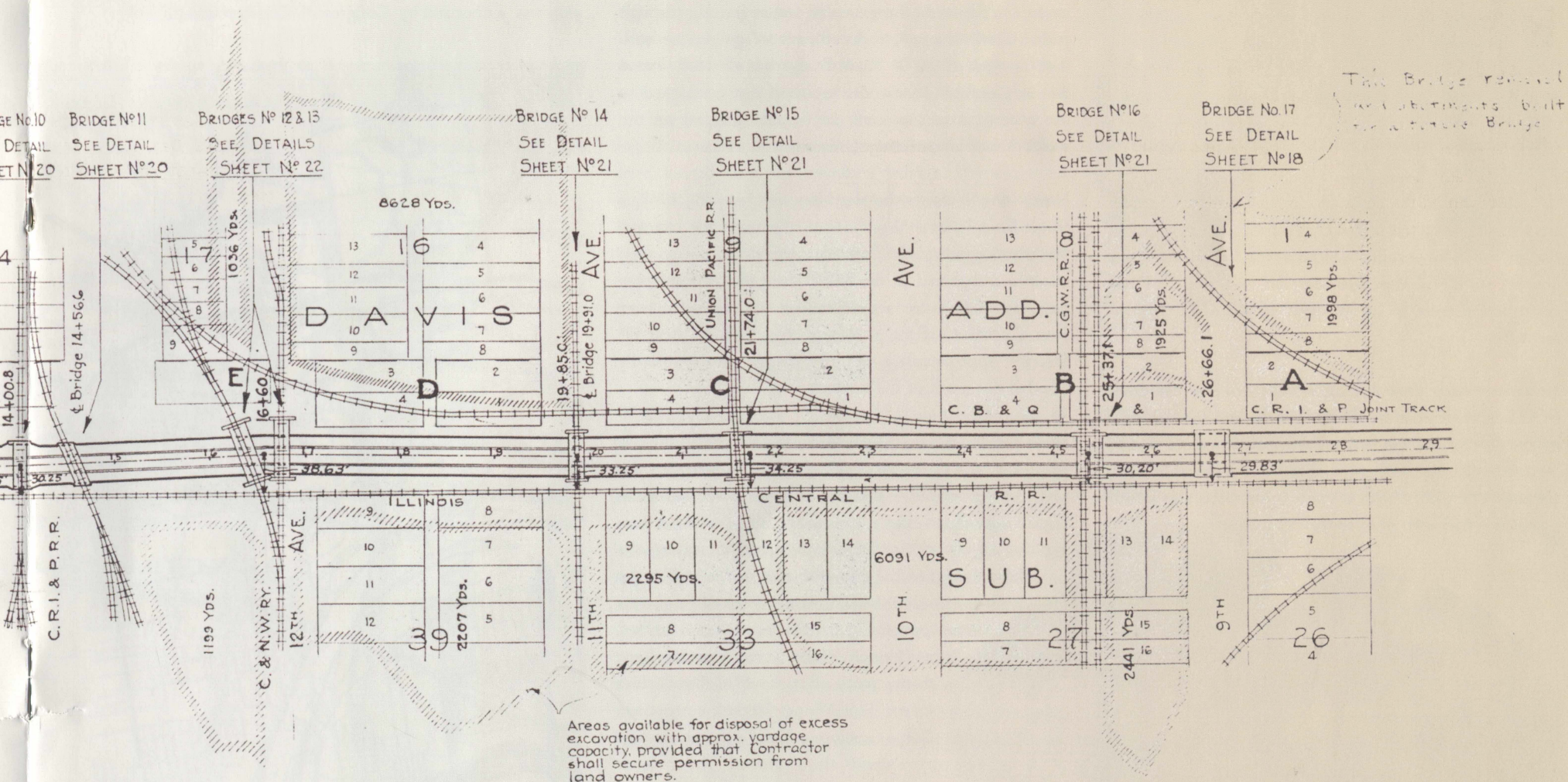
1938 Alvord, Burdick & Howson Engineering Plans for the Indian Creek Channel construction project. Depicted is the channel segment extending adjacent to 14 th Street between 9 th and 16 th avenues (original plans on file at the Department of Public Works, City of Council Bluffs, Iowa).
