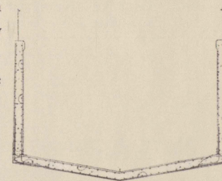
Cross-section schematics of typical 22-foot open (above) and covered (left) concrete channel segments (from Alvord, Burdick & Howson 1938).
