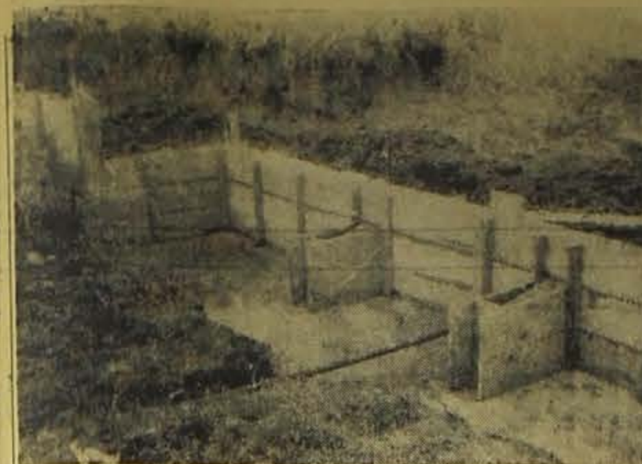
A concrete toe wall structure is shown under construction. The dam was built by Lewis Croser on his farm east of Eldora last fall.
