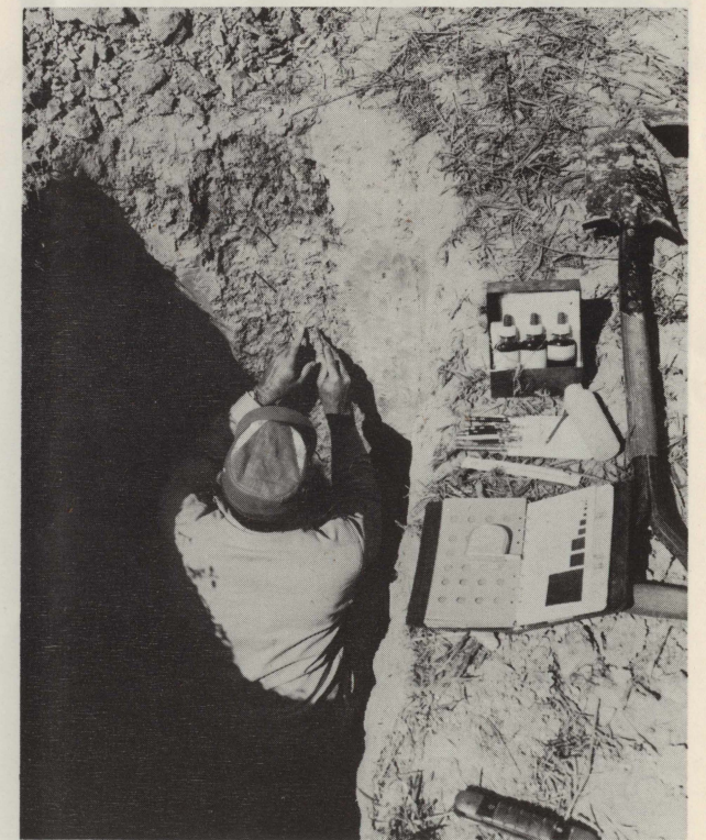
A soil scientist examines the soil layers in a freshly dug pit and describes them in a notebook. The spikes in the bank mark the separate layers.
