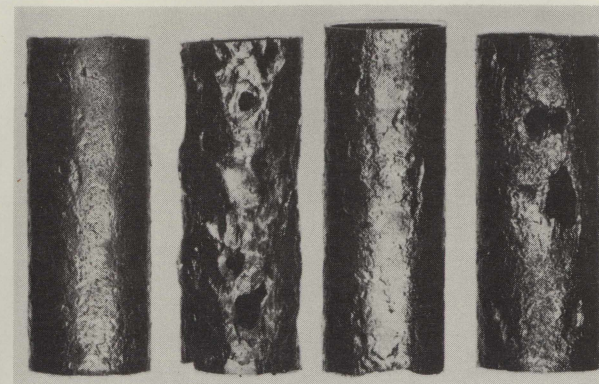
Some soils corrode metal pipes. These steel sections were buried for 14 years in four different kinds of soil. One is almost intact, while the others show different degrees of corrosion.
