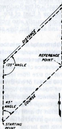
Fig. 1. Sketch of a tract described by the metes and bounds system.
