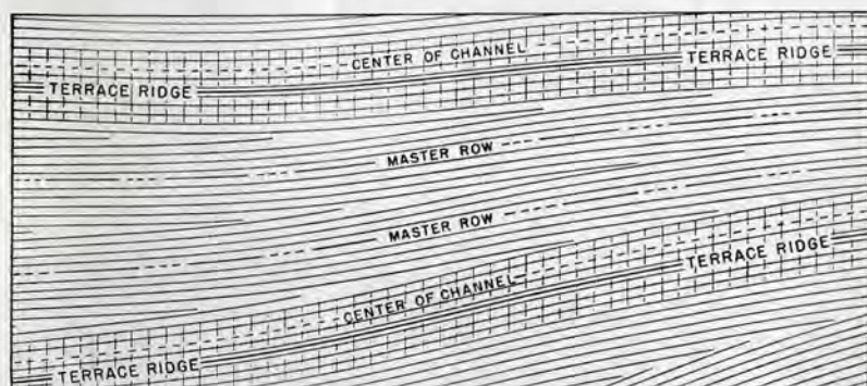
FIGURE 36.—Arranging point rows between master rows on terraced land places all the rows more nearly on the contour than does any of the methods shown in figure 35. This is the most intricate of the four suggested arrangements.
