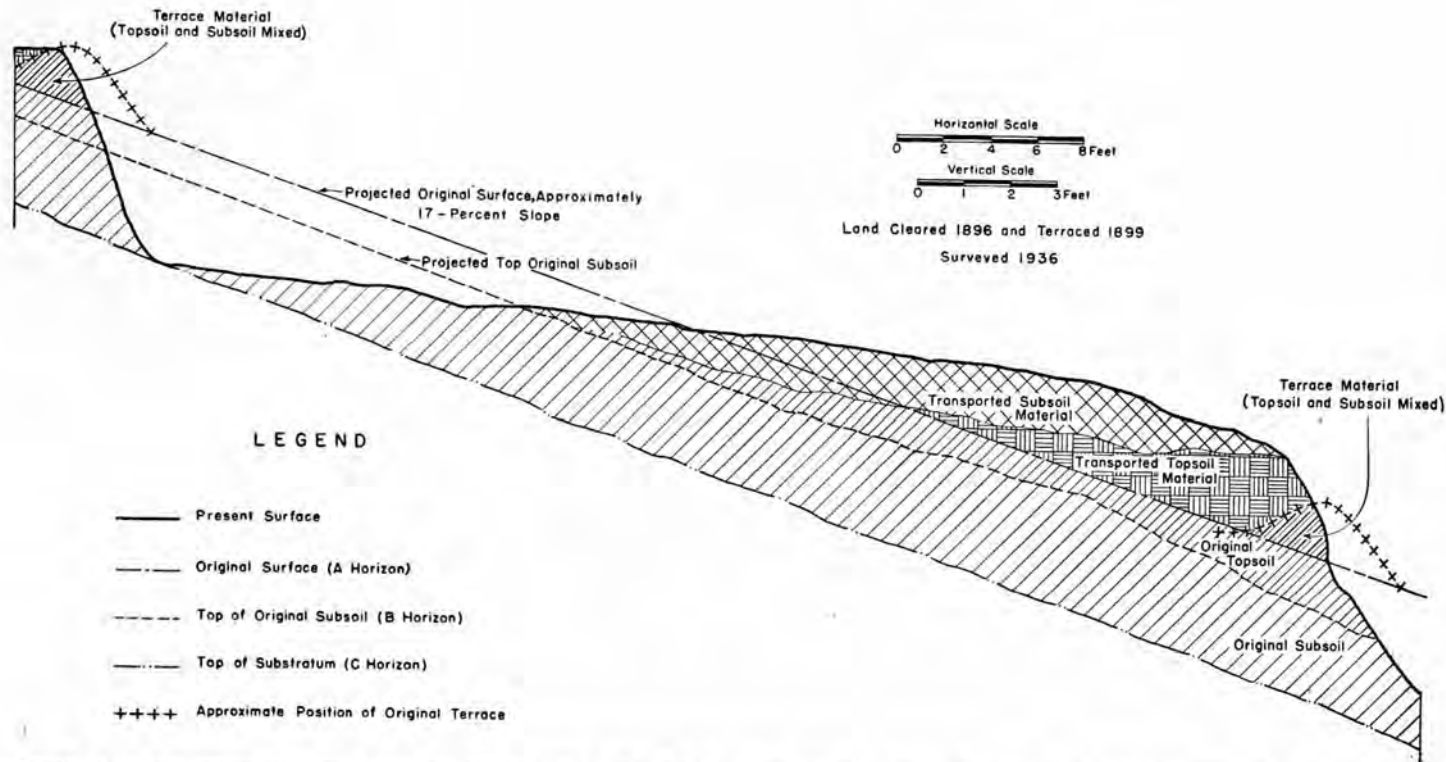
FIGURE 15.—Cross section of a bench terrace. The inverted soil profile has been developed by soil movement between terraces. Unless the topsoil is relatively deep in comparison with the vertical interval between terraces, subsoil is eventually exposed over the entire surface.
