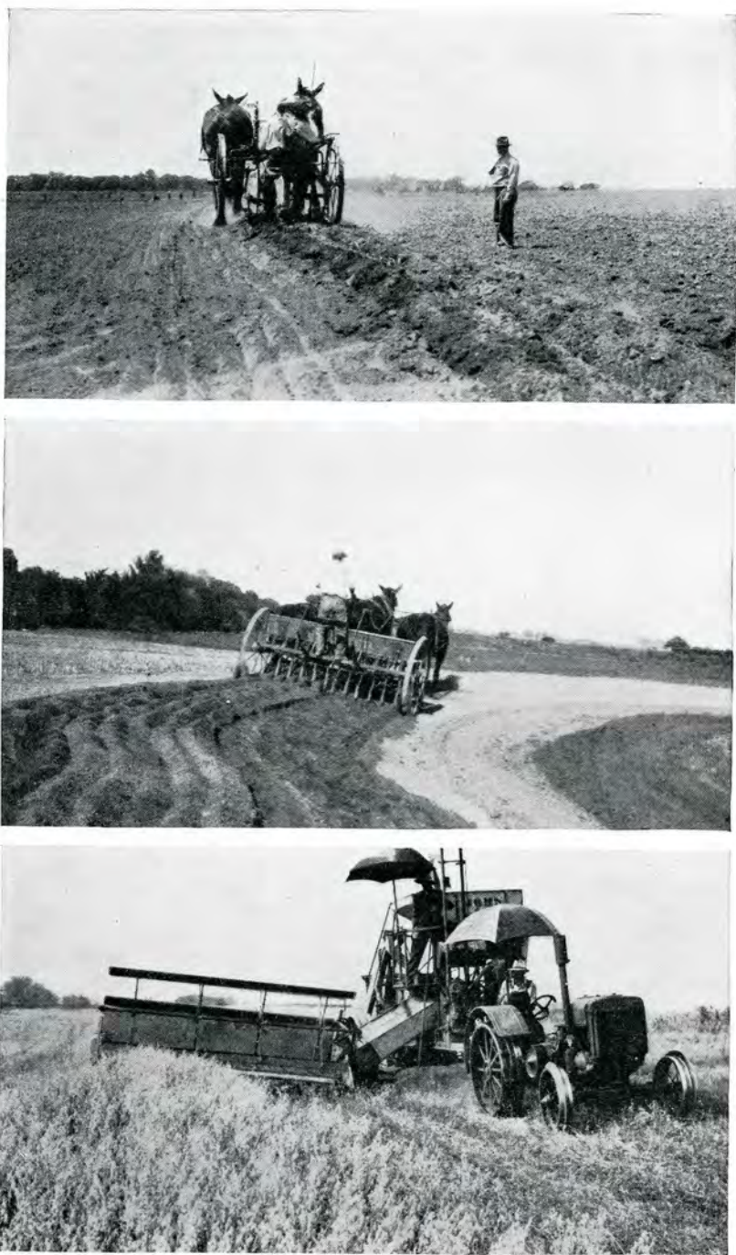
FIGURE 37.—Farm machinery can be satisfactorily operated over terraces if they are properly constructed and if contour tillage is practiced, as shown in the three pictures.
