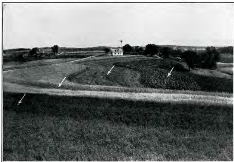
FIGURE 33.—Strip cropping combined with terracing. Adjacent strips are centered on consecutive terraces. The arrows indicate terrace locations.
