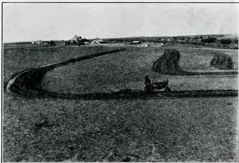
FIGURE 20.—Satisfactory terraces can be constructed with small blade terracers and the regular farm tractor, provided a sufficient number of rounds are made to develop adequate cross sections.
