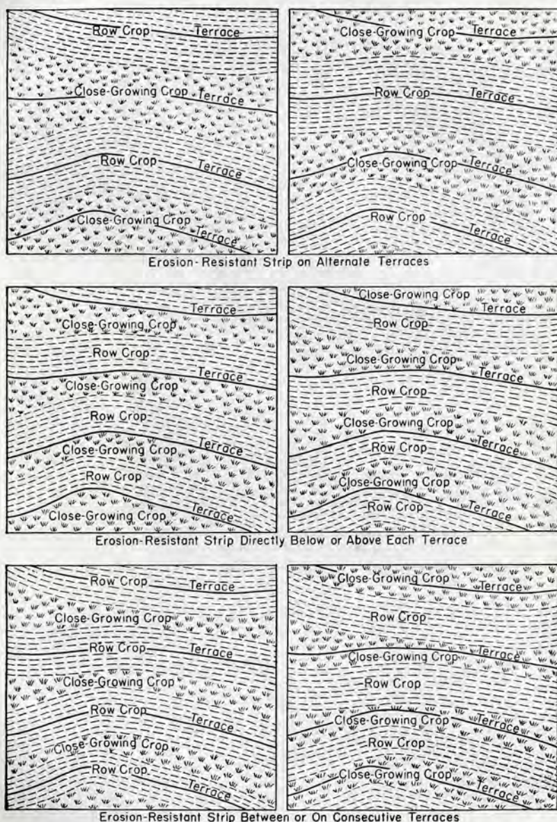
FIGURE 34.—Three suggested methods of combining strip cropping and terracing.
