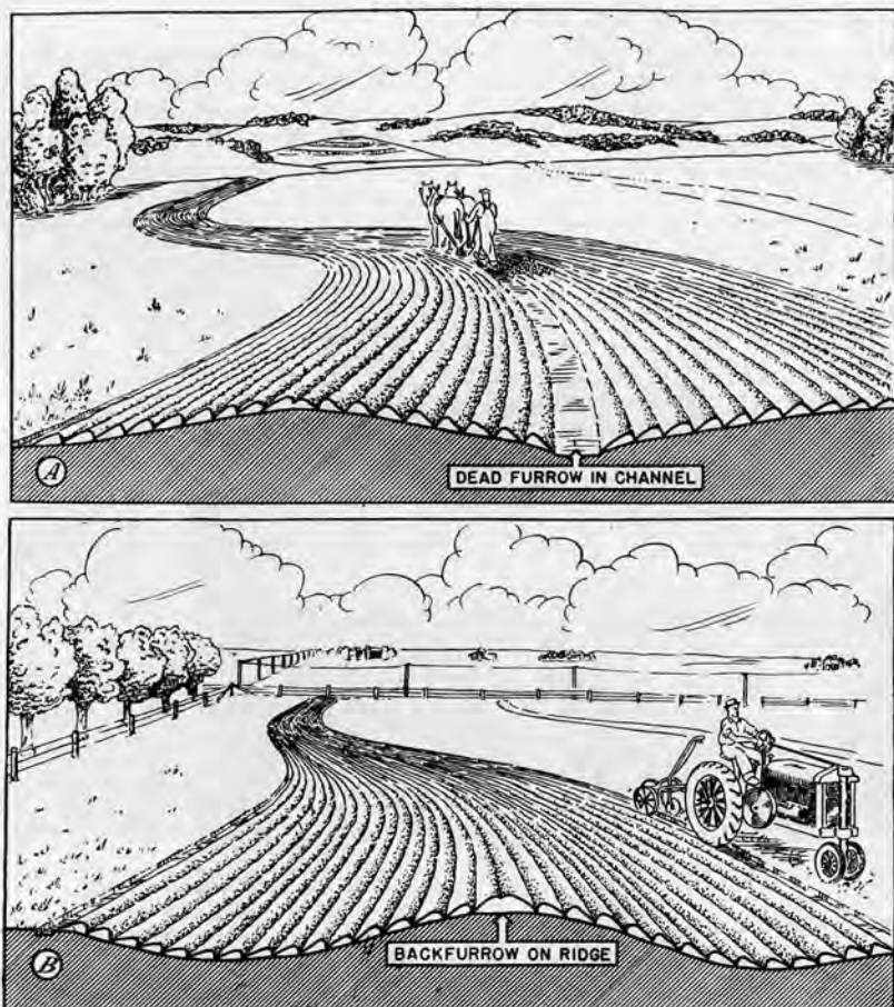
FIGURE 32.—Maintaining terraces by plowing: A, The channel of the drainage-type terrace can be enlarged by plowing it out. Between channels turn as many of the furrows uphill as possible to offset the natural soil movement down the slope. B, The ridge of the absorptive-type terrace can be enlarged by backfurrowing to it. The location of the dead furrow should be varied from year to year to avoid excessive depression at any one point.
