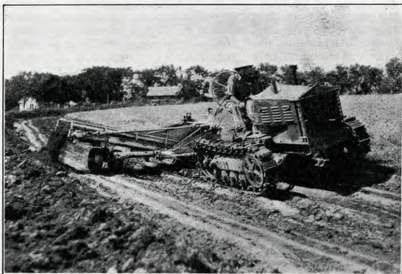
FIGURE 23.—The elevating grader-type terracer developed by the Agricultural Engineering Department of the University of Missouri.
