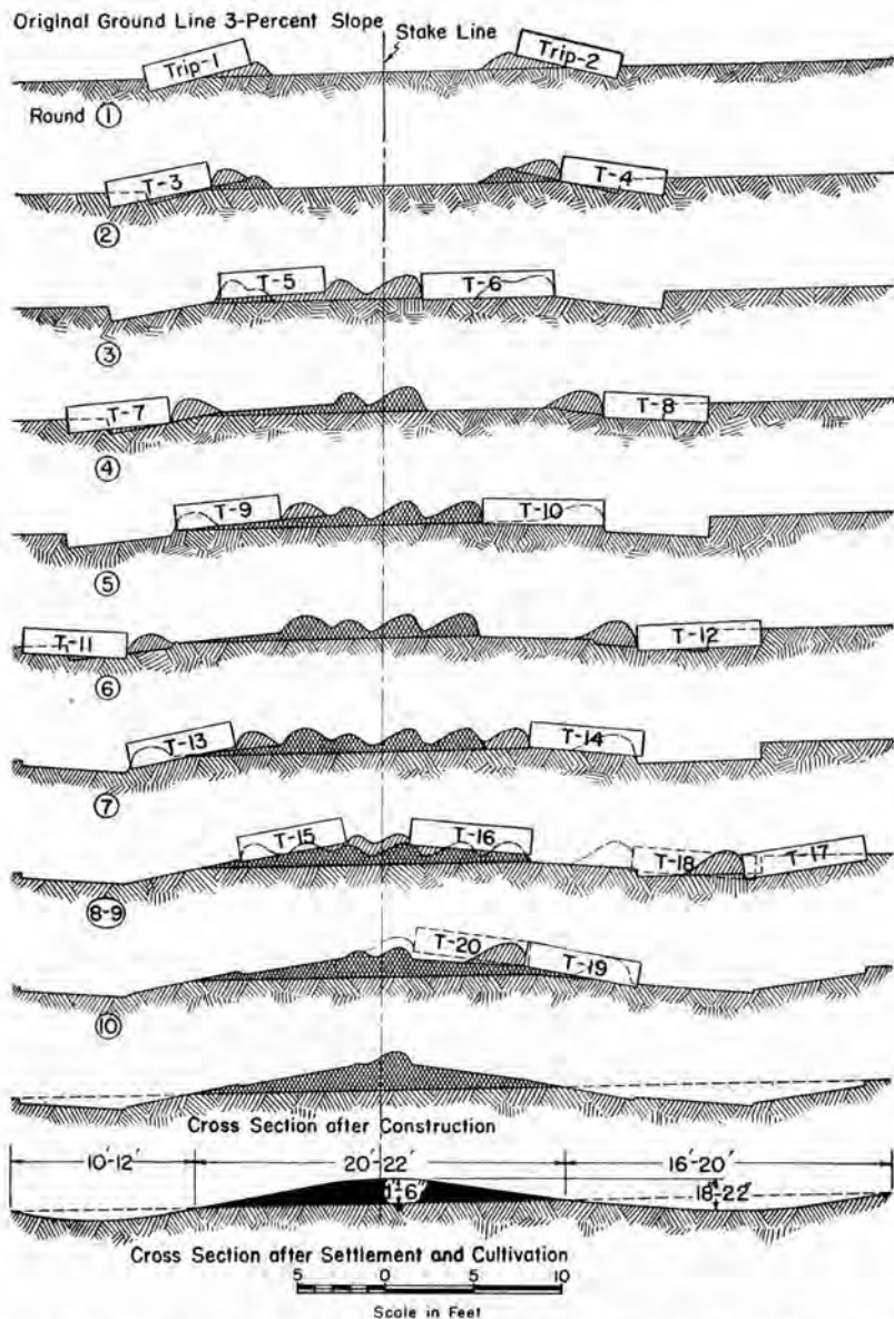
FIGURE 26.—Progressive steps in constructing an absorptive-type terrace in the Great Plains with a 10-foot blade terracer. The terrace is constructed from both sides. With inexperienced operators and on certain soil types it may be desirable to secure the necessary center height during the first few rounds.
