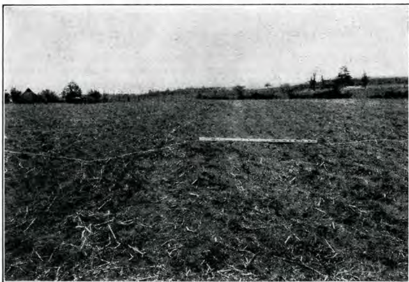
FIGURE 11.—This drainage-type terrace has been blended into the surface slopes and the channel capacity maintained by proper plowing. The terrace will offer a minimum of inconvenience to tillage operations.
