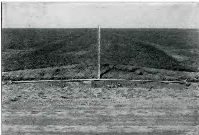
FIGURE 12.—The absorptive-type terrace is used in the Great Plains for erosion control and moisture conservation. It is important that the ridge be high enough to spread the collected run-off over a wide area and wide enough to allow satisfactory operation of tillage equipment.
