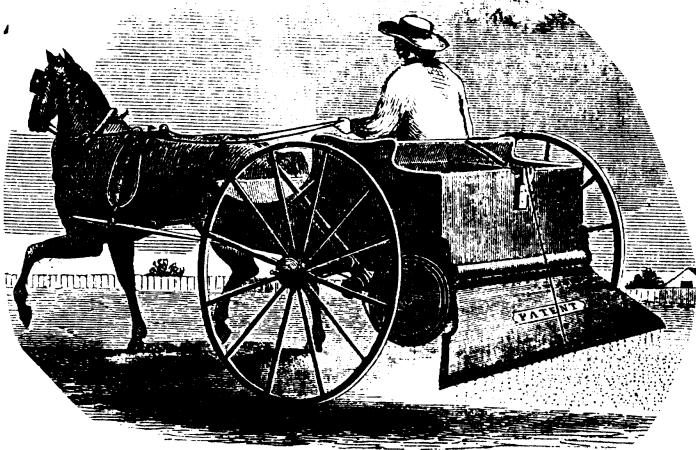
Stevens' Broadcast Seed Sower. [Patented May 22, 1855.]
